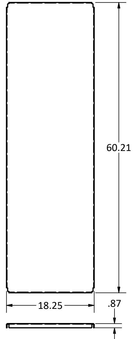
5' TAMARACK LOG HOLDER STEEL LID
