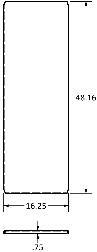
4' TAMARACK LOG HOLDER STEEL LID
