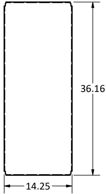
3' TAMARACK LOG HOLDER STEEL LID
