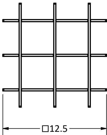
SMALL FIRE GRATE
